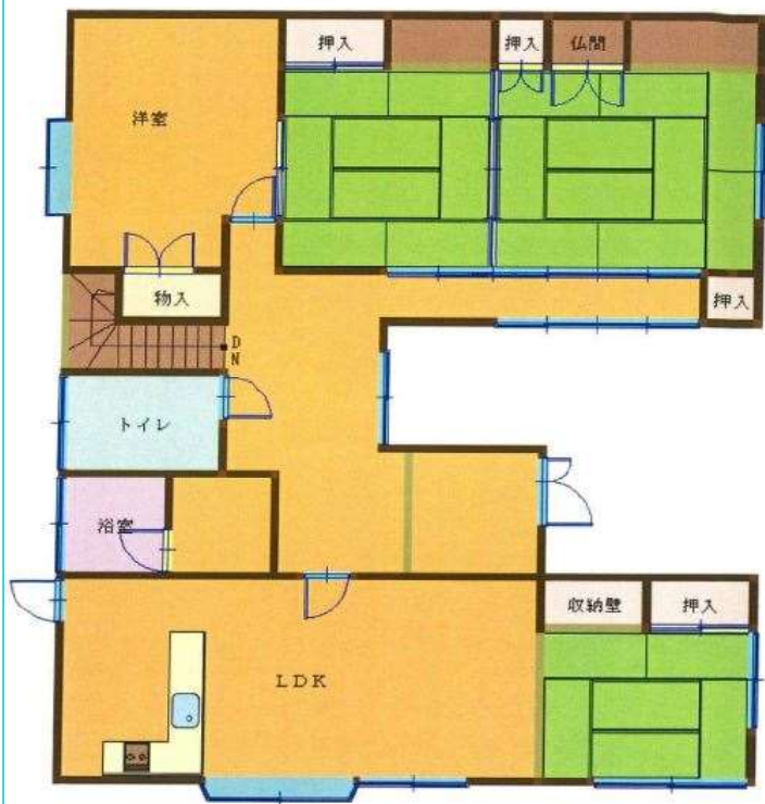
1F
